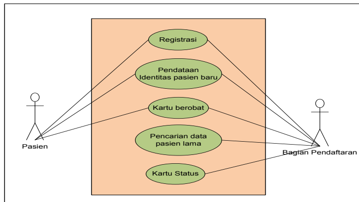
Gambar 4.14 Use Case Diagram Proses Pendaftaran
