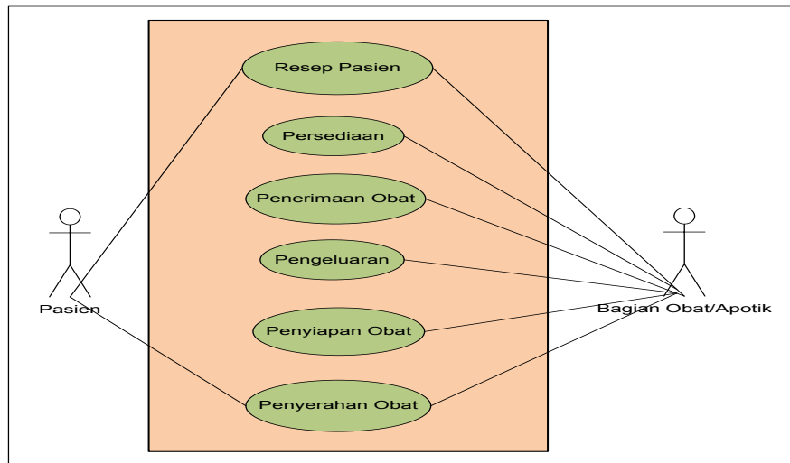
Gambar 4.16 Use Case Diagram Proses Pelayanan Obat
